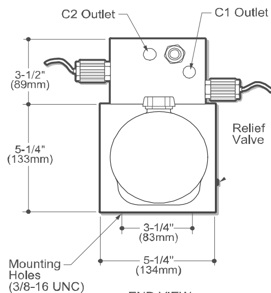
END VIEW
