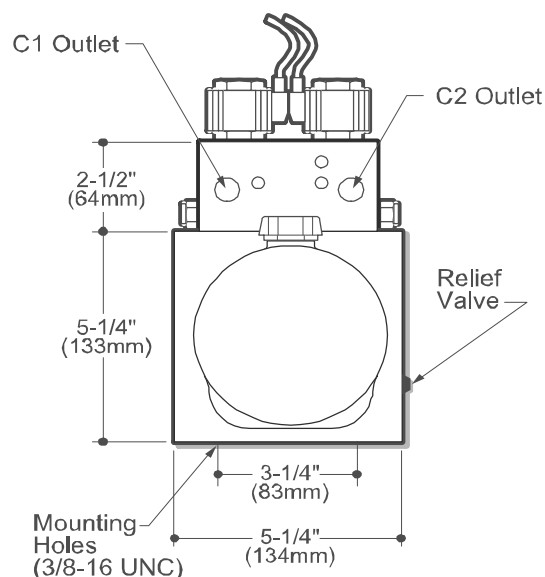
END VIEW
