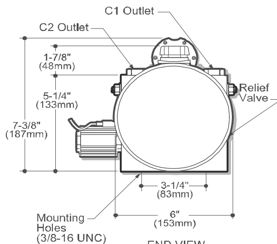
END VIEW
