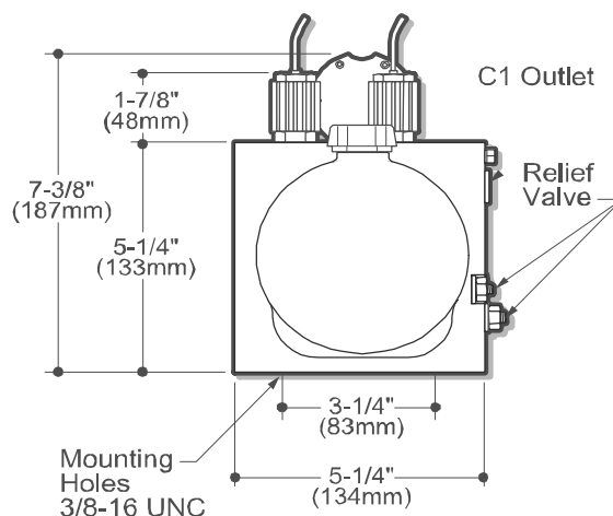
END VIEW
