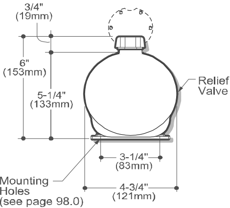
END VIEW
