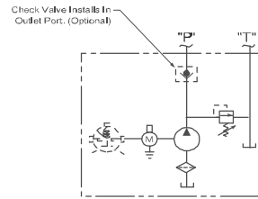
M-3598 HYDRAULIC SCHEMATIC
