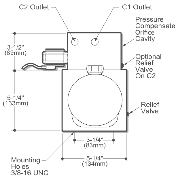
END VIEW
